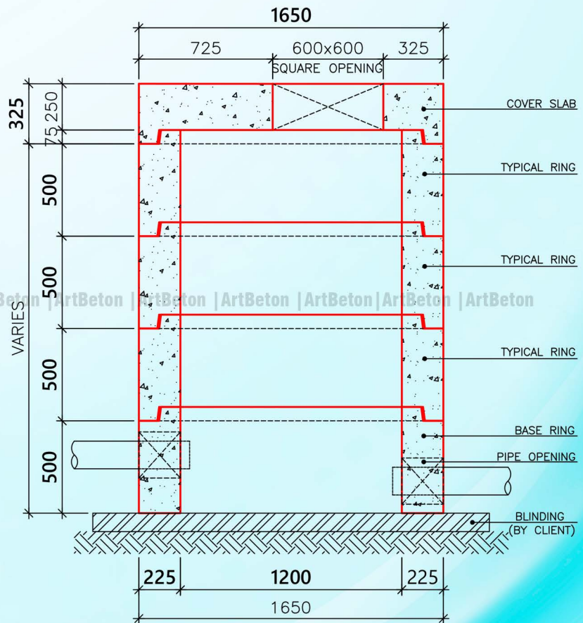
01 MH RING 1200 DIA --- SCALE
